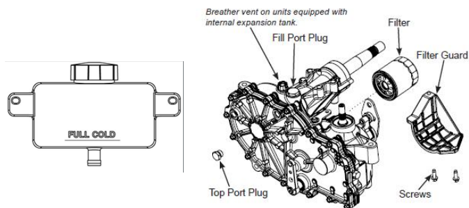
Figure 6, Unit With Internal Expansion Tank
